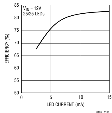
Conversion Efficiency
