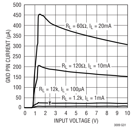
GND Pin Current LT3009-1.2
