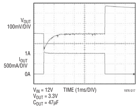
LT1976 No Load 1A Step Response
