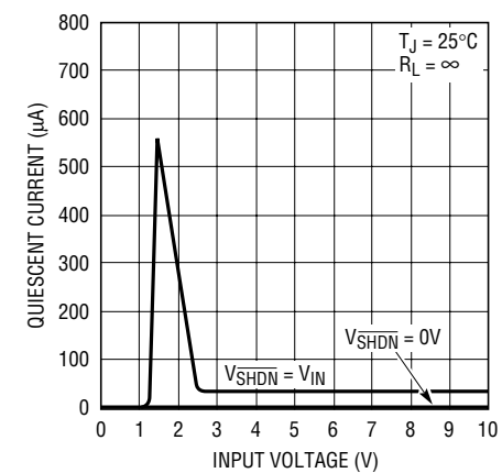
LT1962-2.5 Quiescent Current
