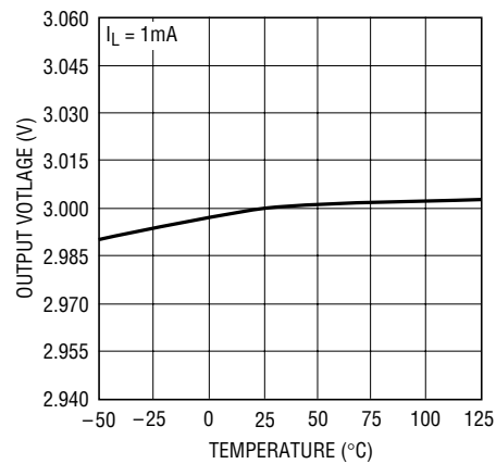
LT1962-3 Output Voltage
