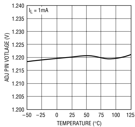
LT1962 ADJ Pin Voltage
