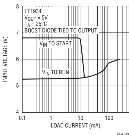
Figure 3. The Minimum Input Voltage Depends on Output Voltage, Load Current and Boost Circuit
