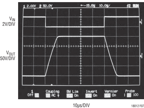
Figure 7. Large-Signal Time Domain Response of the Amplifier
