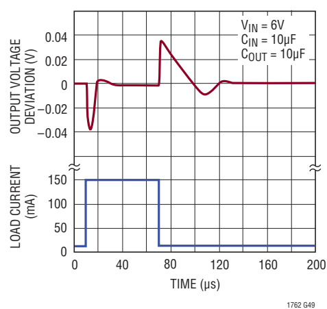
LT1762-5 Transient Response C_{BYP} = 0.01 \mu F
