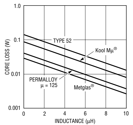
Inductor Core Loss for 3.3V Output
