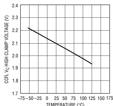
CCFL V C High Clamp Voltage vs Temperature
