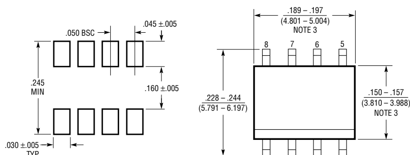
RECOMMENDED SOLDER PAD LAYOUT
