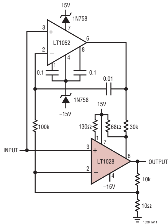
Chopper-Stabilized Amplifier
