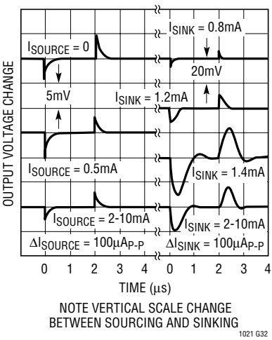
Load Transient Response LT1021-10, C_{LOAD} = 1000pF
