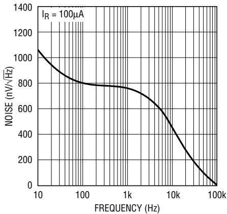
Noise Voltage
