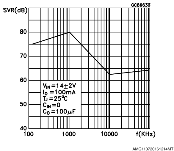
Figure 20. Supply voltage rejection vs frequency
