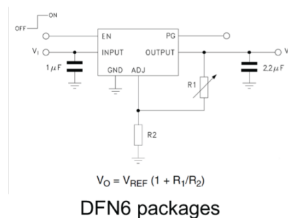
Figure 4. Adjustable version (PPAK and DFN6 packages only)
