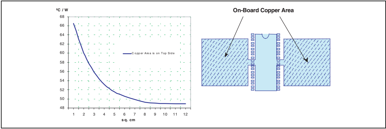
Figure 29. Mounting the PowerSO Package.
