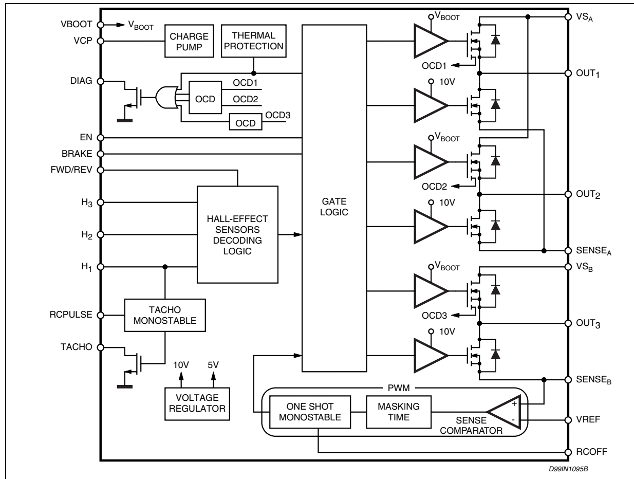
Figure 2. Block Diagram
