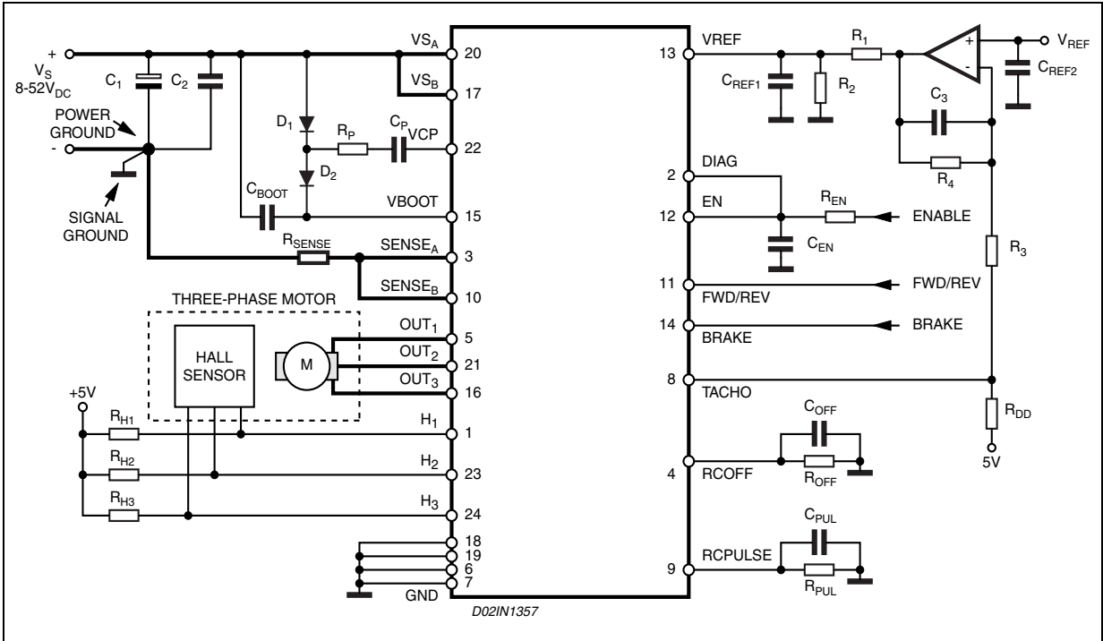
Figure 24. Typical Application
