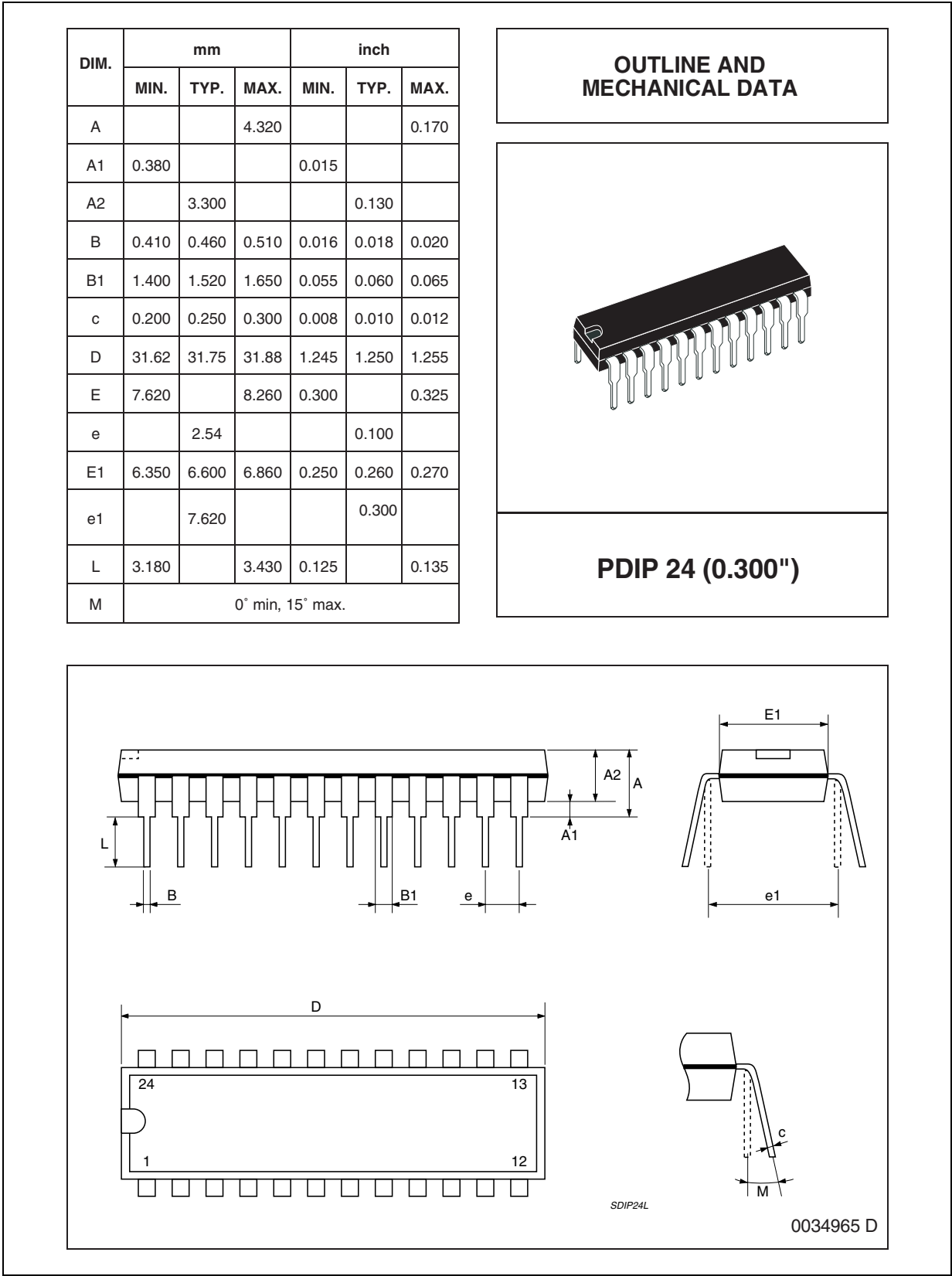
Figure 31. PDIP-24 Mechanical Data & Package Dimensions
