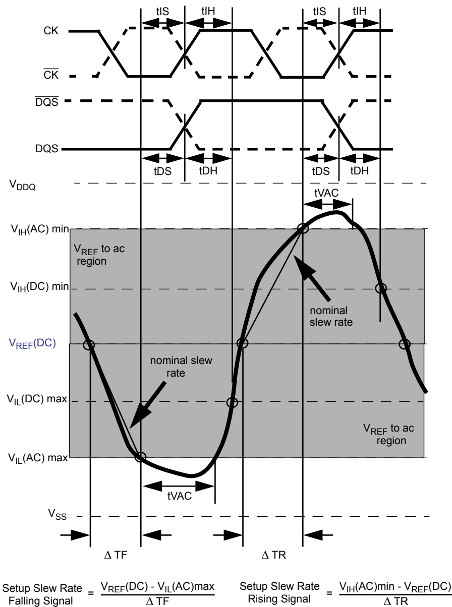
Figure 21. Illustration of nominal slew rate and t_{VAC} for setup time t_{DS} (for DQS with respect to strobe) and t_{IS} (for ADD/CMD with respect to clock).
