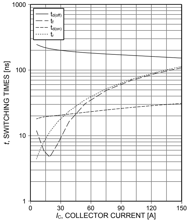
Figure 8. Typical switching times as a function of collector current (inductive load, T_{vj}=150^\circ\text{C} , V_{CE}=400\text{V} , V_{GE}=15/0\text{V} , r_G=12\Omega , Dynamic test circuit in Figure E)
