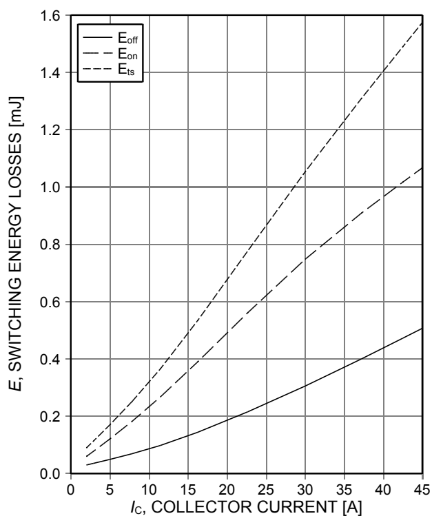
Figure 12. Typical switching energy losses as a function of collector current (inductive load, T_{vj}=150^\circ\text{C} , V_{CE}=400\text{V} , V_{GE}=15/0\text{V} , r_G=39\Omega , Dynamic test circuit in Figure E)
