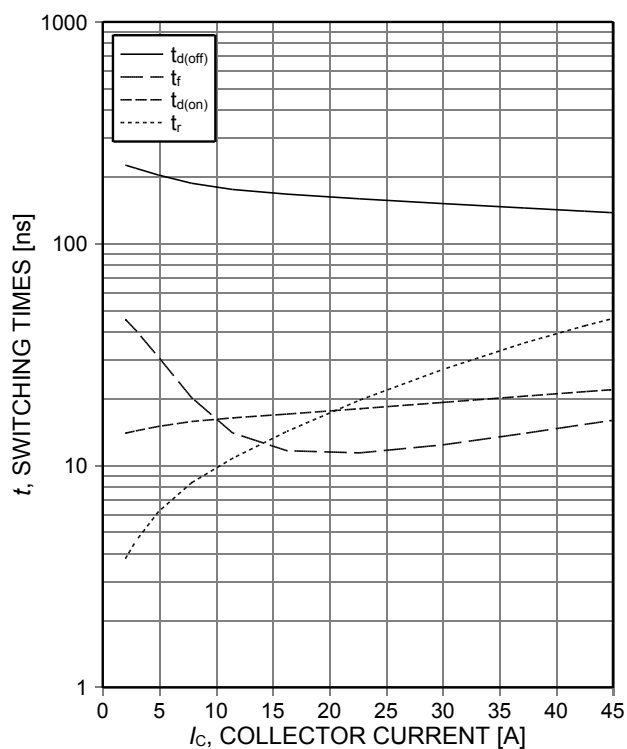
Figure 8. Typical switching times as a function of collector current (inductive load, T_j=150^\circ\text{C} , V_{CE}=400\text{V} , V_{GE}=15/0\text{V} , r_G=39\Omega , Dynamic test circuit in Figure E)
