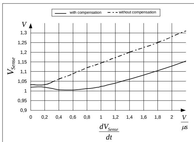
Figure 15 Overcurrent Shutdown
