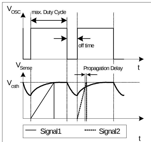
Figure 16 Dynamic Voltage Threshold V_{csth}
