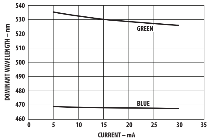
Figure 6: Dominant Wavelength vs. Forward Current (InGaN Devices)
