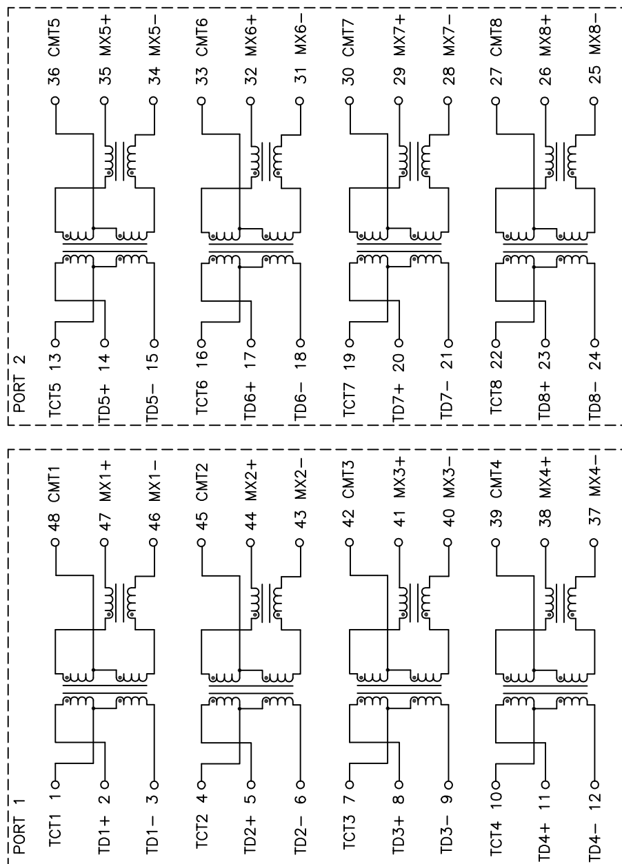
SCHEMATIC
