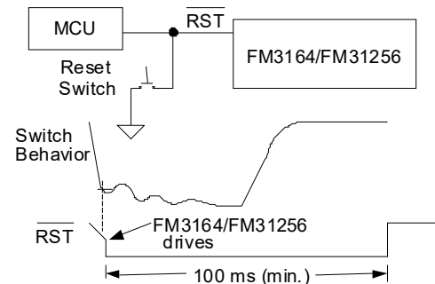
Figure 4. Manual Reset
