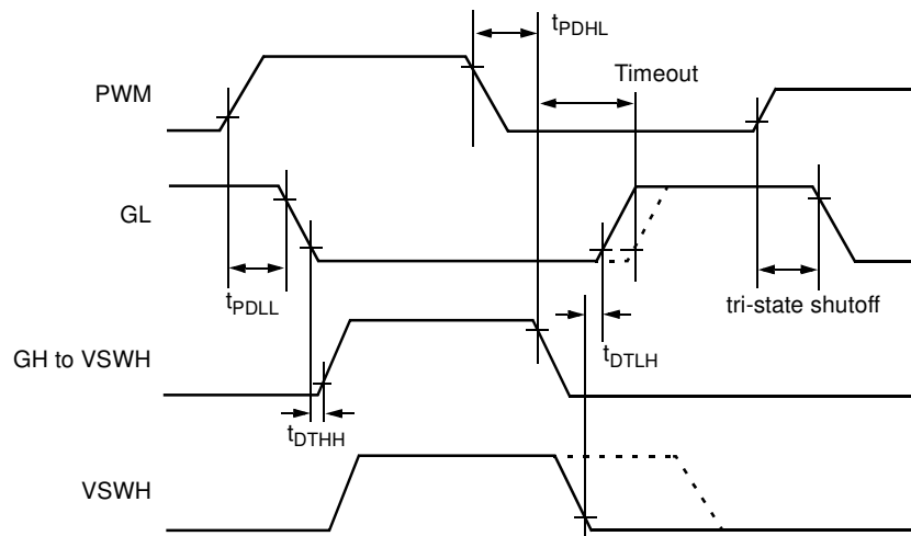
Figure 4. Timing Diagram
