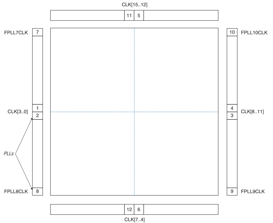
Figure 2–40. PLL Locations
