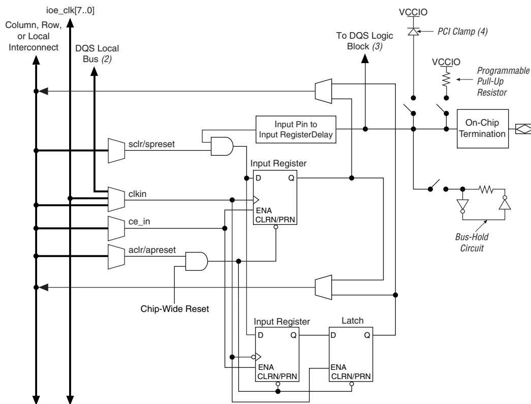
Figure 2–52. Stratix II IOE in DDR Input I/O Configuration Notes (1), (2), (3)
