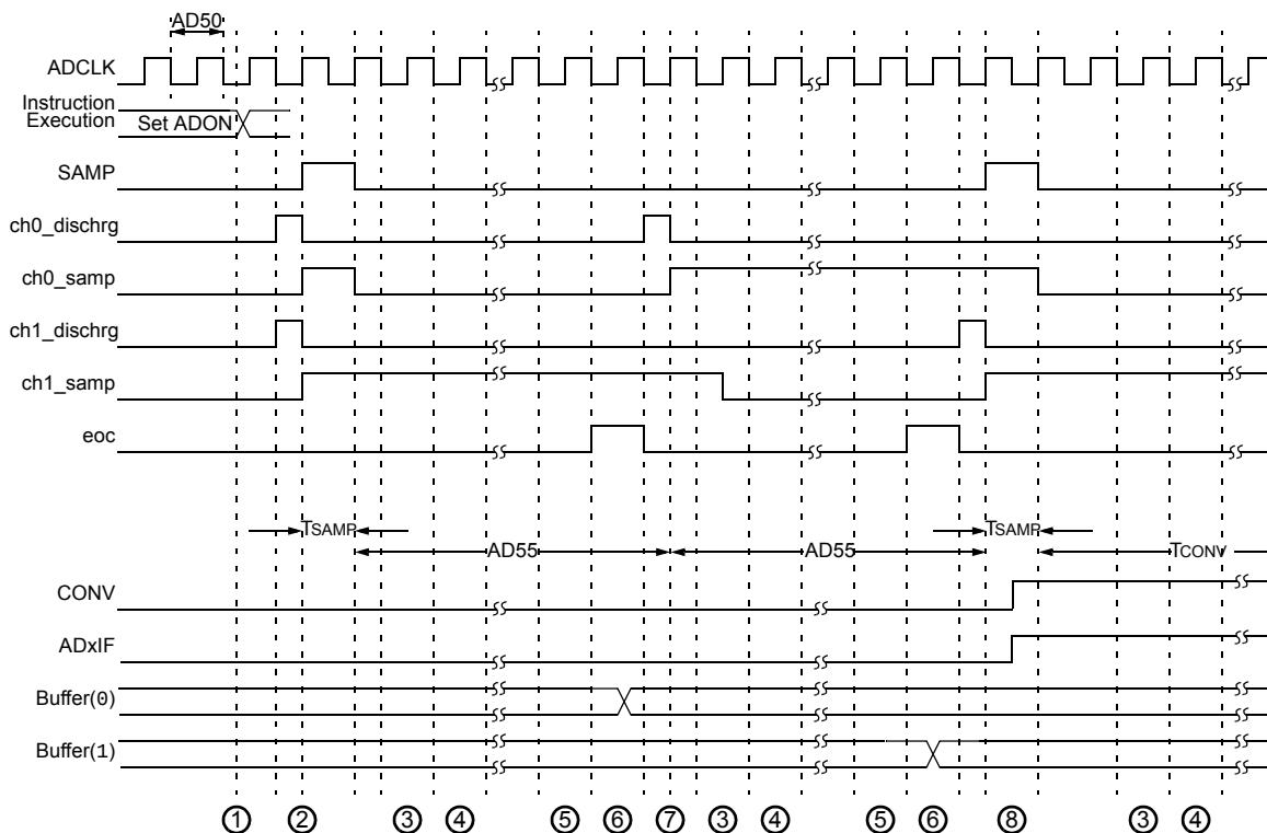
FIGURE 26-29: ADC CONVERSION (10-BIT MODE) TIMING CHARACTERISTICS (CHPS<1:0> = 01, SIMSAM = 0, ASAM = 1, SSRC<2:0> = 111, SAMC<4:0> = 00001)
