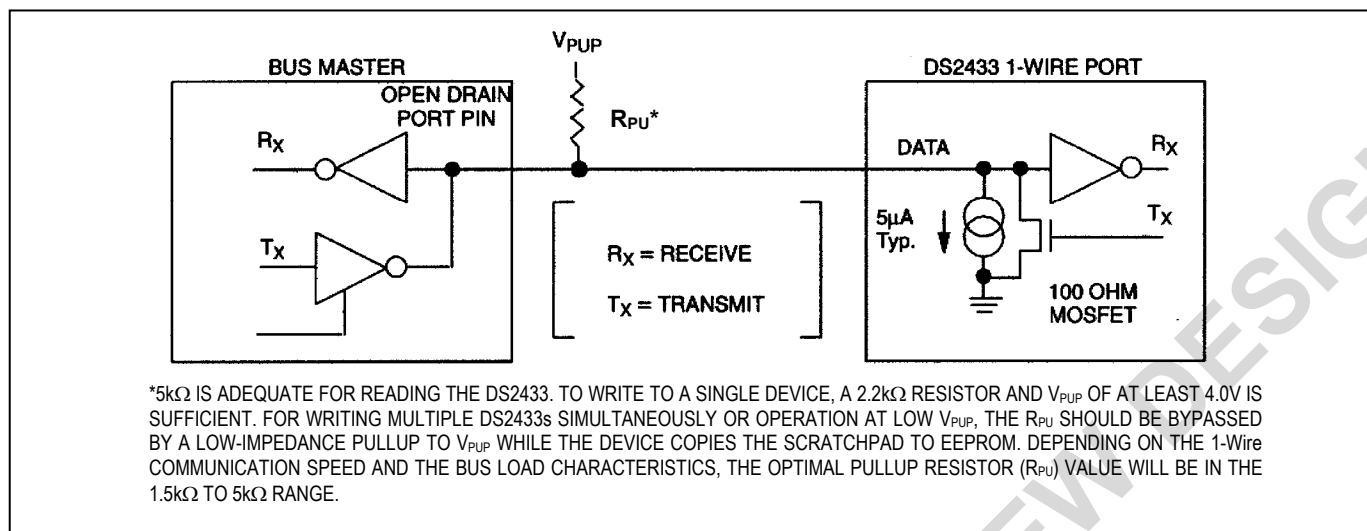
Figure 8. HARDWARE CONFIGURATION
