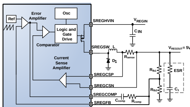
Figure 5-4. Built-in Switching Regulator
