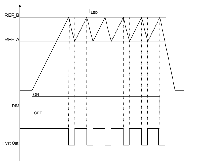
Figure 5-2. Current Waveforms
