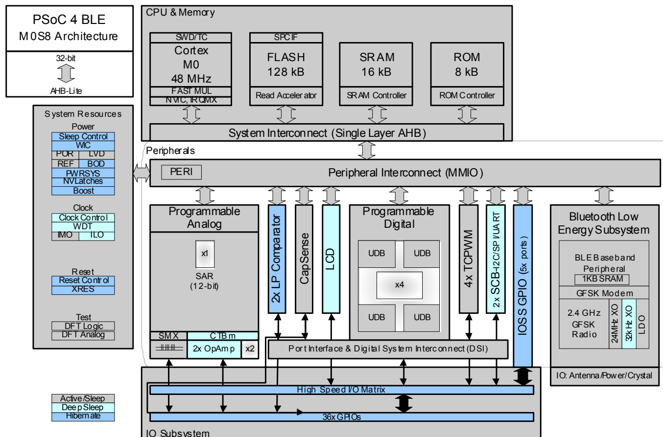
Figure 2. Block Diagram
