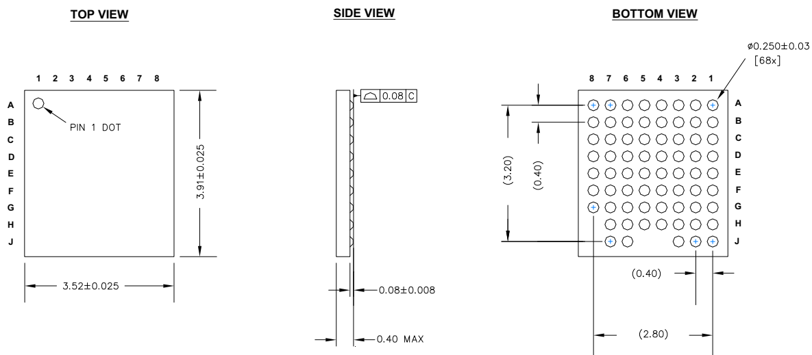
Figure 10. 68-Ball Thin WLCSP
