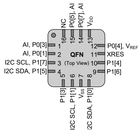
Figure 5. CY8C21223 16-Pin QFN
