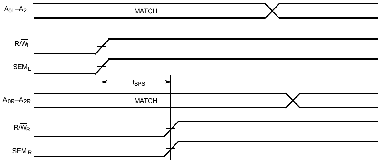
Figure 10. Timing Diagram of Semaphore Contention [42, 43, 44]
