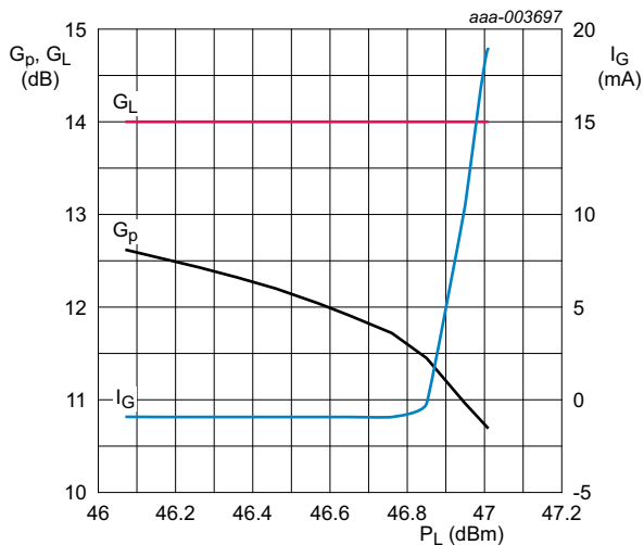
Fig 5. Power gain, linear gain and gate current as function of output power; typical values
