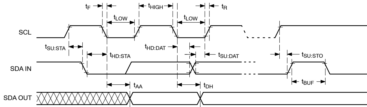
Figure 5. Bus Timing
