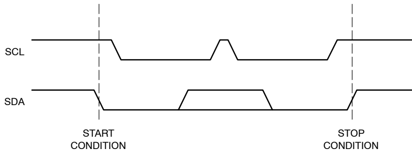
Figure 2. START/STOP Conditions
