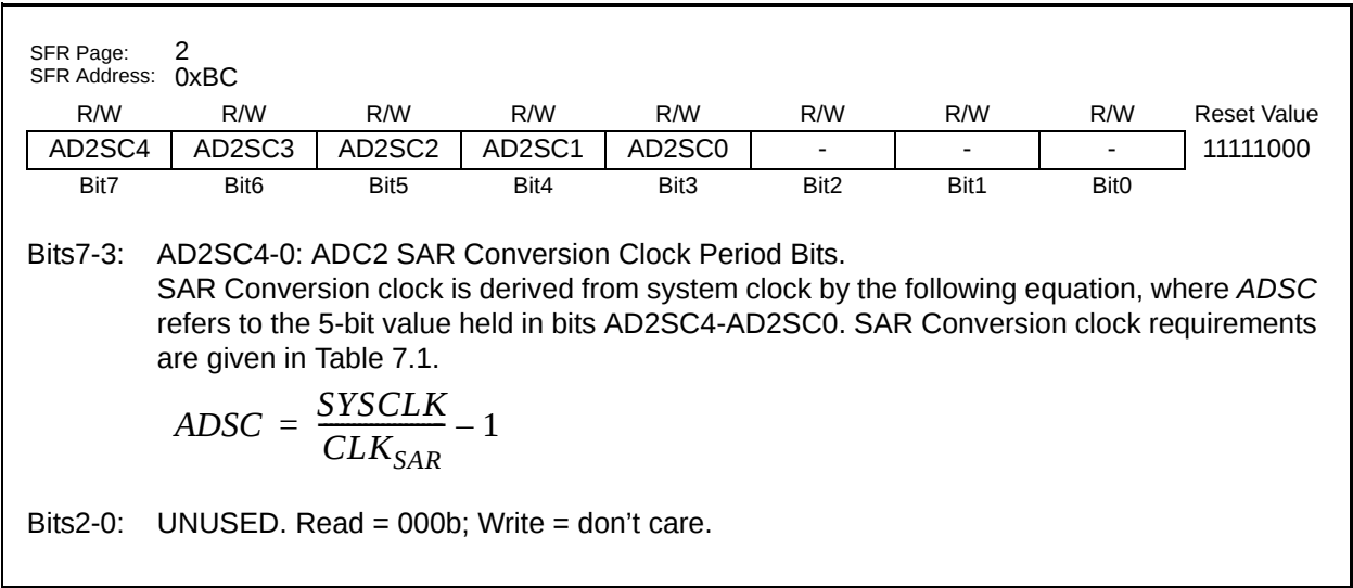
Figure 7.7. ADC2CF: ADC2 Configuration Register
