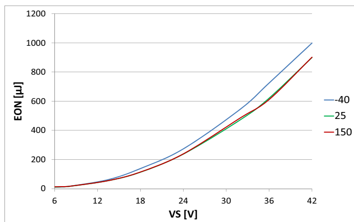
Figure 40 Switch ON Energy E_{ON} = f(T_J; V_S) , R_L = 6 \Omega
