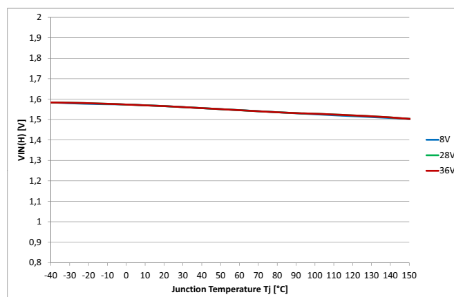
Figure 49 Input Voltage Threshold V_{IN(H)} = f(T_J; V_S)
