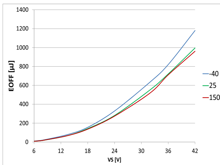
Figure 41 Switch OFF Energy E_{OFF} = f(T_J; V_S) , R_L = 6 \Omega
