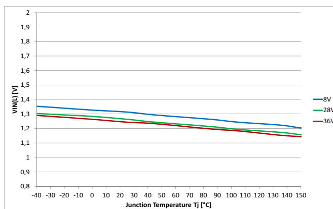
Figure 48 Input Voltage Threshold V_{IN(L)} = f(T_J; V_S)
