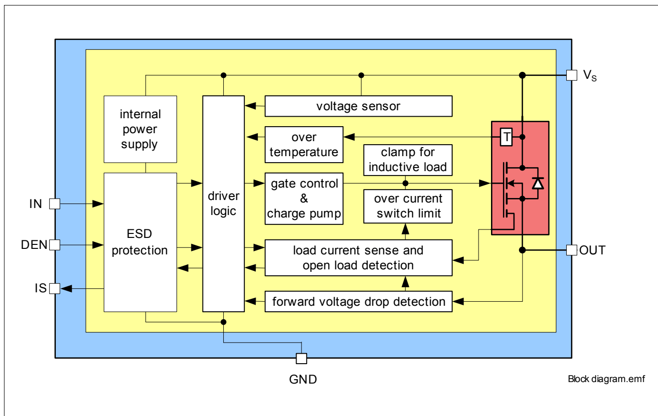
Figure 1 Block Diagram for the BTT6020-1EKA
