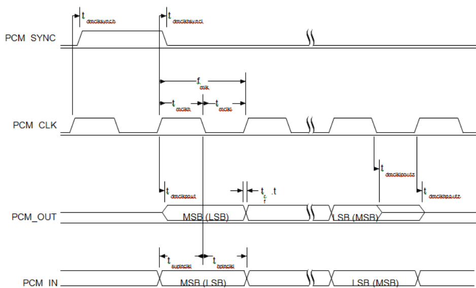
Figure 10: PCM Master Timing Short Frame Sync
