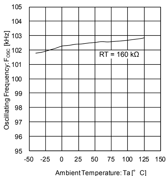
Figure 3. Oscillating Frequency vs Temperature (RT=160kΩ)
