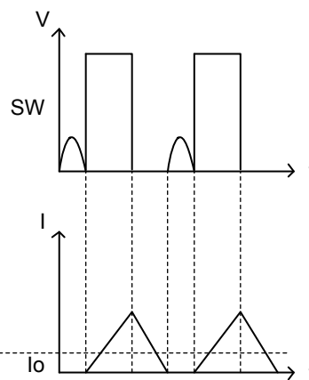
Figure 21. Discontinuous Action
