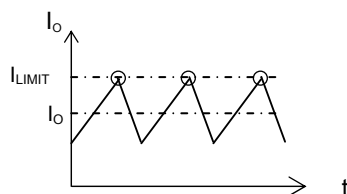
Figure 22. Overcurrent Detection
