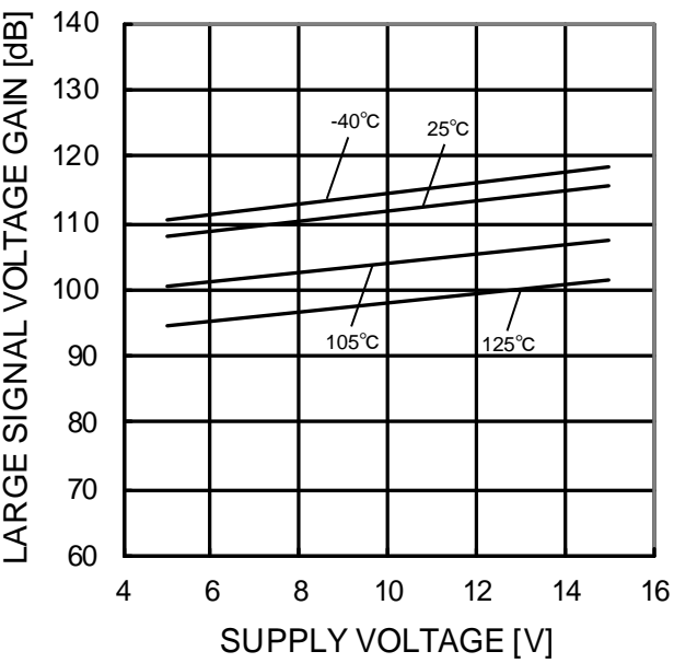
Figure 69. Large Signal Voltage Gain - Supply Voltage (R L =2kΩ)
