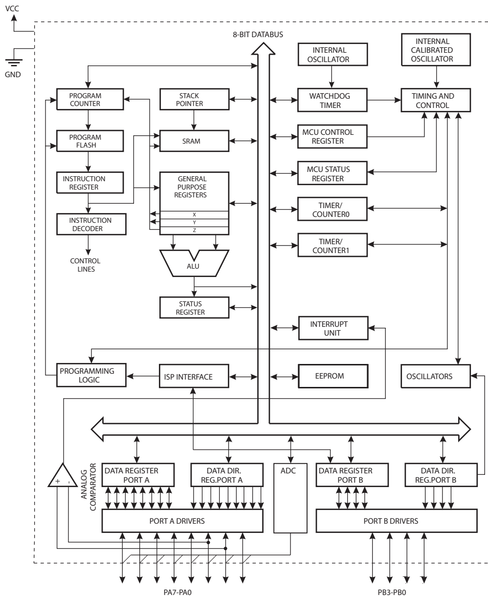
Figure 2-1. Block Diagram
