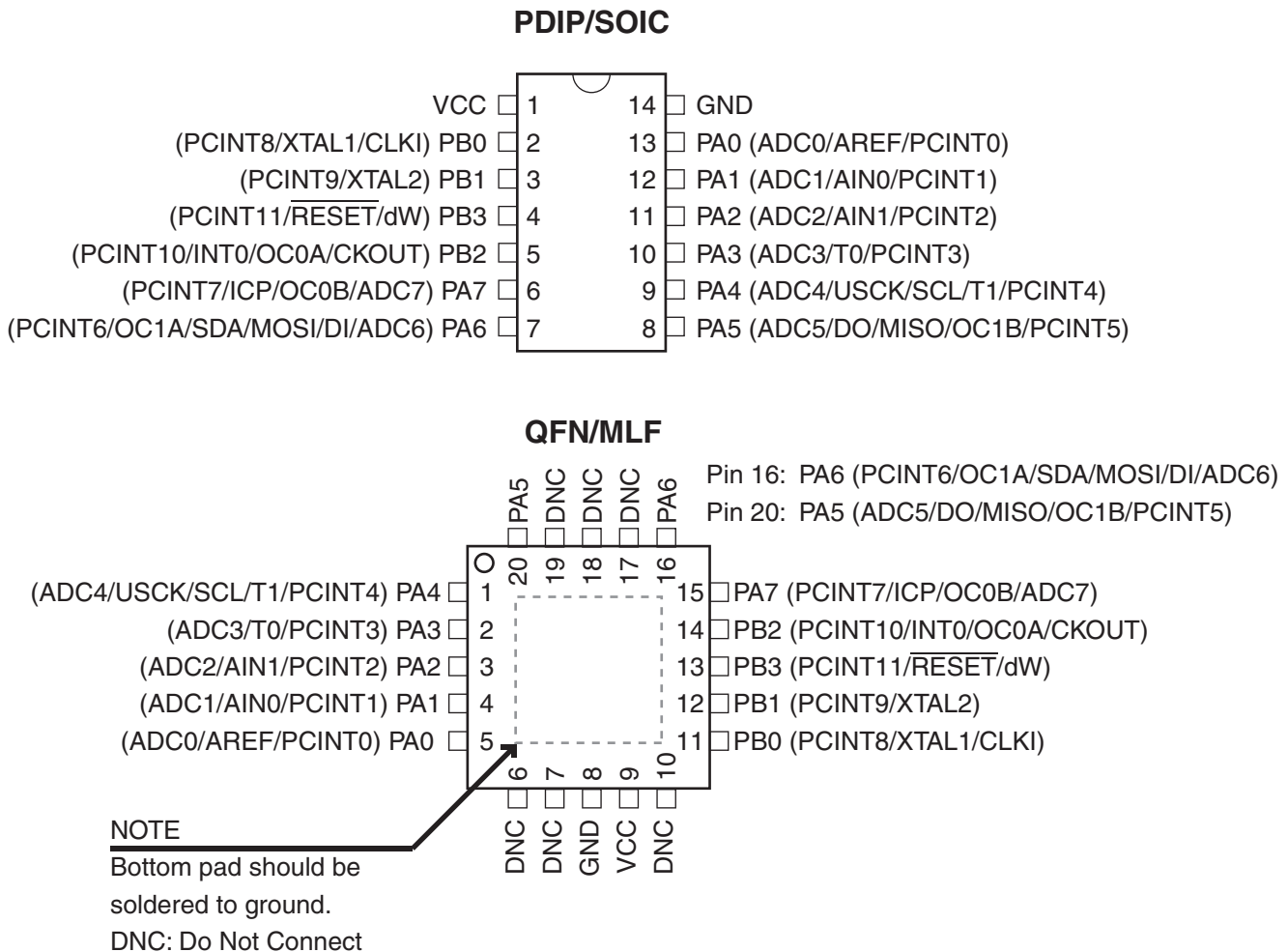
Figure 1-1. Pinout ATtiny24/44/84
