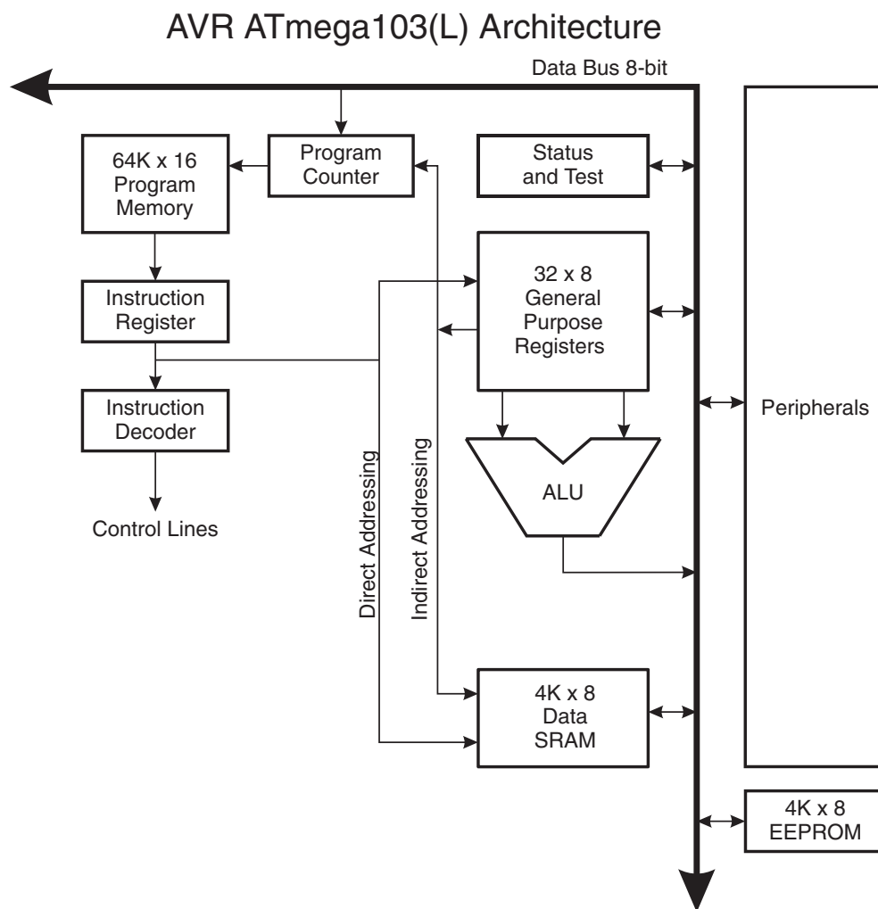
Figure 4. The ATmega103(L) AVR RISC Architecture
