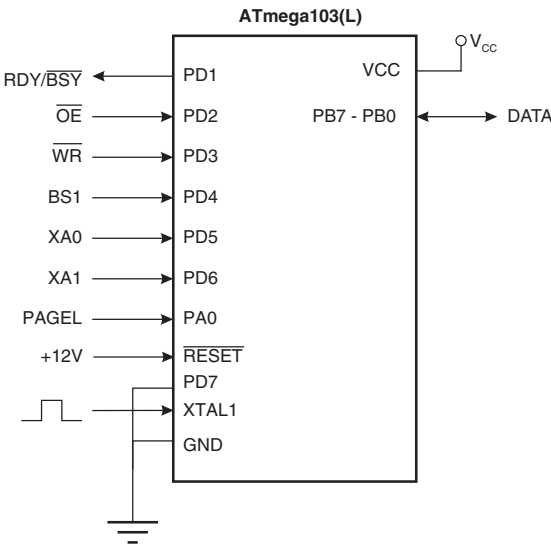
Figure 72. Parallel Programming
