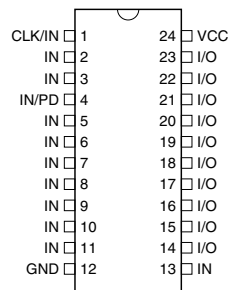
Figure 2-2. DIP/SOIC
