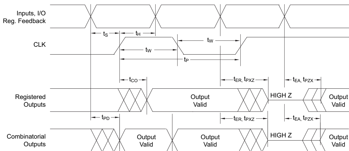
Figure 3-2. AC Waveforms
