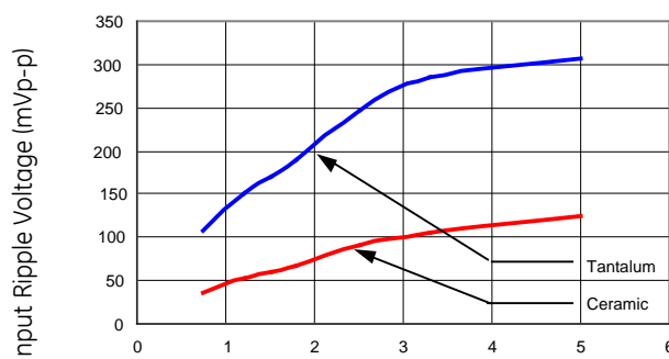
Figure 27. Input ripple voltage for various output with 2x47 μF tantalum capacitors and with 2x22 μF ceramic capacitors at the input (80% of I_{O,max} ).
