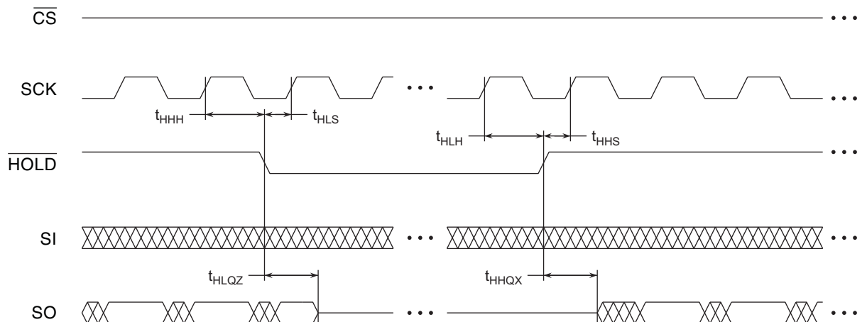
Figure 16-5. \overline{\text{HOLD}} Timing – Serial Output
