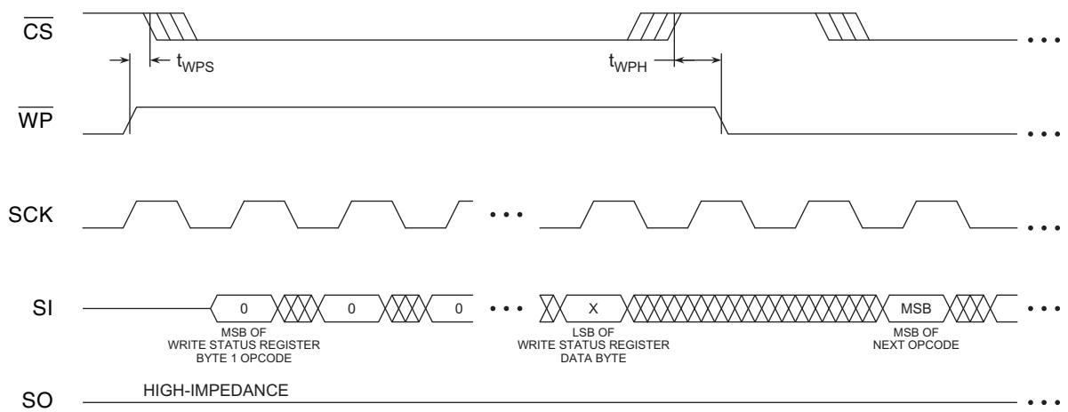
Figure 16-3. \overline{\text{WP}} Timing for Write Status Register Byte 1 Command When SPRL = 1
