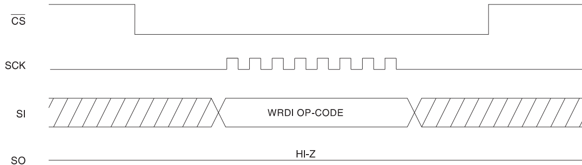
Figure 5. WRDI Timing
