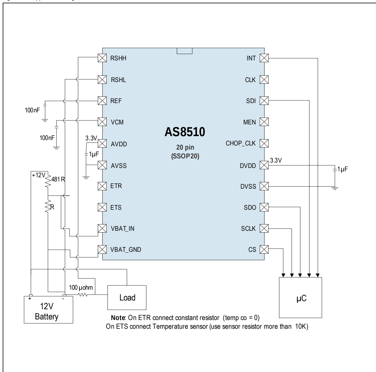
Figure 20. Application Diagram
