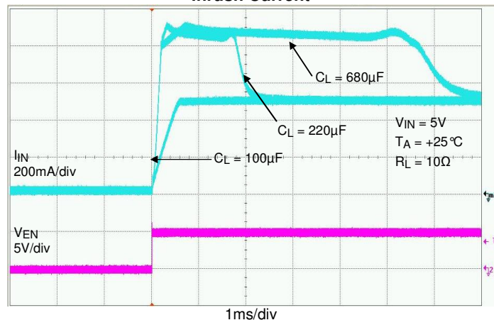
Inrush Current
