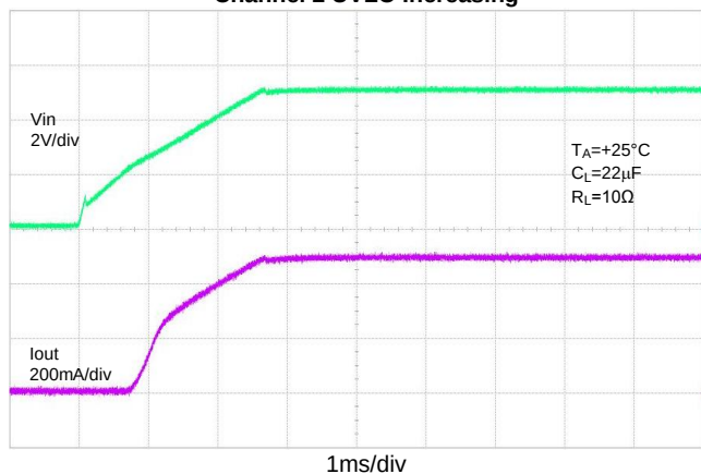
Channel 2 UVLO Increasing
