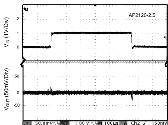
Line Transient (Condition: V_{IN}=2.5\text{V} to 3.5\text{V} , I_{OUT}=10\text{mA} )
