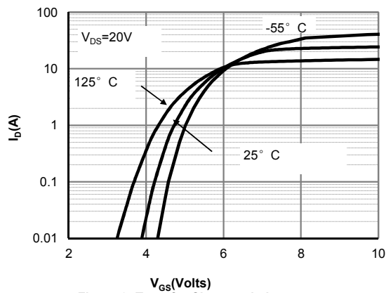
Figure 3: Transfer Characteristics
